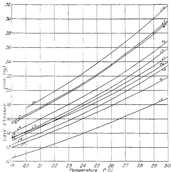
Fig. 1.—Vapor pressures of saturated aqueous solutions. (1) \text{NH}_4\text{Cl} ; (2) \text{NH}_4\text{NO}_3 ; (3) (\text{NH}_4)_2\text{SO}_4 ; (4) \text{NH}_4\text{H}_2\text{PO}_4 ; (5) \text{NH}_4\text{Cl} + \text{KNO}_3 ; (6) \text{KCl} ; (7) \text{KNO}_3 ; (8) \text{NaNO}_3 ; (9) Urea; (10) \text{H}_2\text{O} (Scheele and Heuse).
